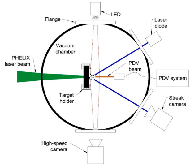
Fig. 3. Schematic of the online diagnostics used during the experimental campaign.
