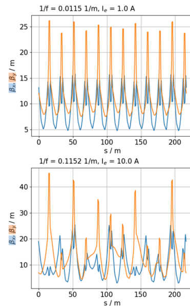
Figure 4: Optical functions at presence of a single electron lens with 1 A (top) and 10 A (bottom) electron beam current in sector 10 of SIS18.
