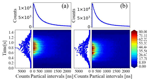
Figure 9: Simulated particle interval distributions of spills extracted with (a, beam size = 3.1 mm) and without (b, beam size = 4.9 mm) emittance exchange.
