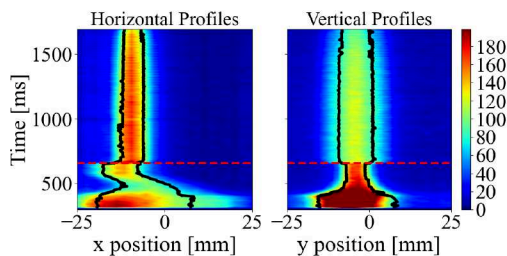
Figure 1: Beam size evolution at horizontal and vertical plane in one acceleration cycle when emittance exchange was executed. The black lines represent the standard deviation of the beam profiles with respect to the beam centers.
