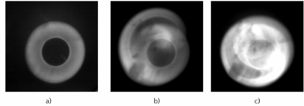
Figure 6: CHROMOX measurements of a 7 keV hollow electron beam: a) 2 mA b) 44 mA c) 87 mA
