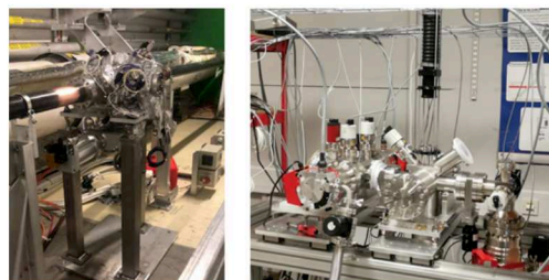
Figure 3: The LHC installation of the interaction chamber (on the left) and the CI assembly (on the right).
