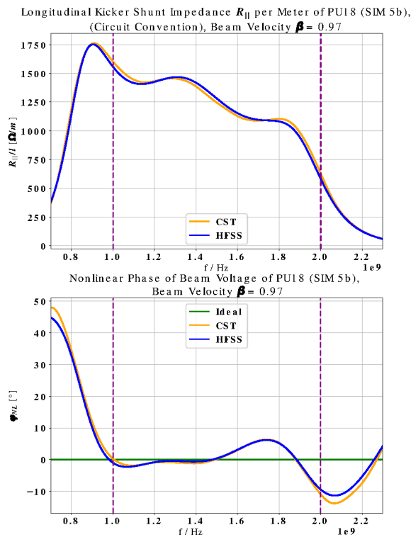
Figure 3: Comparison between CST and HFSS.
