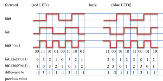
Figure 3: Evaluation of the stepping motor pulses to reveal the sense of rotation.
