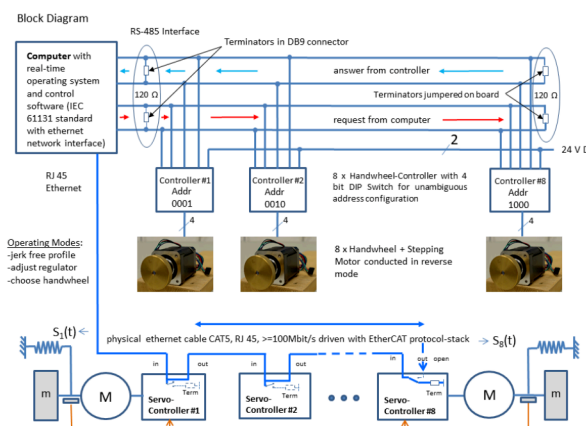
Figure 1: Linear drive control scheme for CR stochastic cooling pickup tanks, supplemented by eight addressable rotary encoders, attached to a four-wire RS-485 bus.
