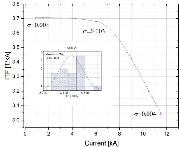
Figure 6: Current dependence of Integral transfer functions of the quadrupoles. The inset graph gives the distribution for 22 series magnets at 900 A.
