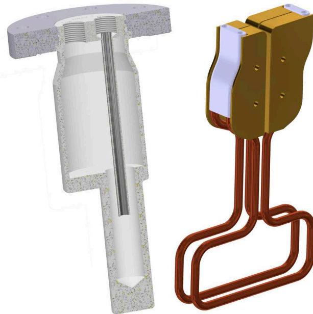
Figure 5: Left: Mechanical design of the static frequency plungers. Right: Mechanical design of the coupling loop.
