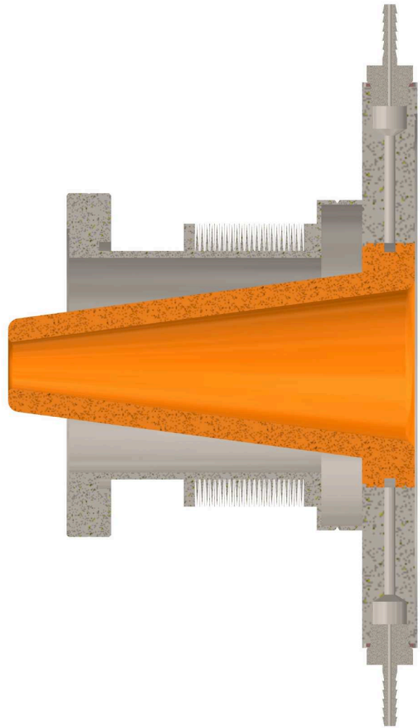
Figure 6: Cut view of the beam catcher cone.
