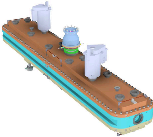
Figure 3: Digital Mockup of the Ladder RFQ including the subcomponents RF coupler, motor driven frequency plungers and the cooling system.
