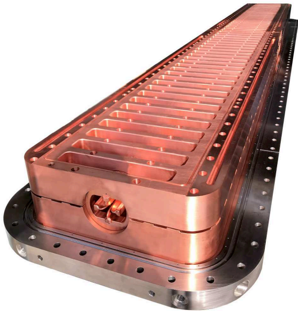
Figure 4: RF ladder structure during assembly and before closing the tank.
