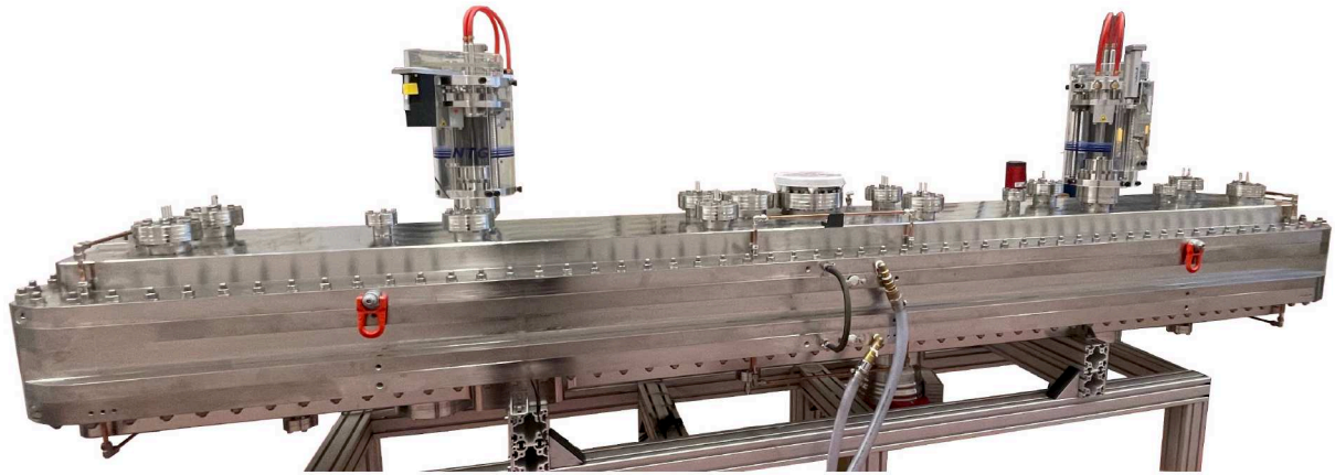
Figure 2: Photo of the Ladder RFQ including assemblies: 10 static frequency plungers, 2 movable frequency plungers and the cooling system.
