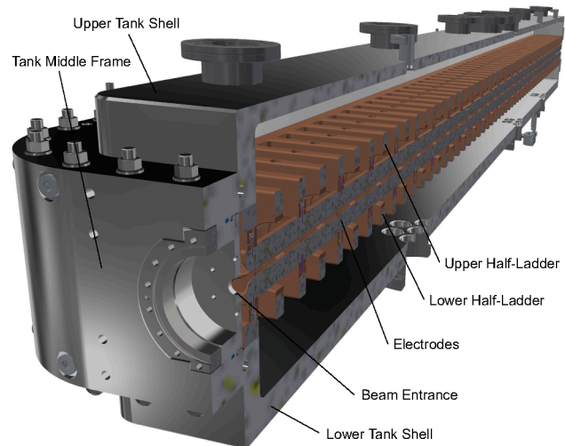
Figure 1: Cut view of the Ladder RFQ showing the individual components.
