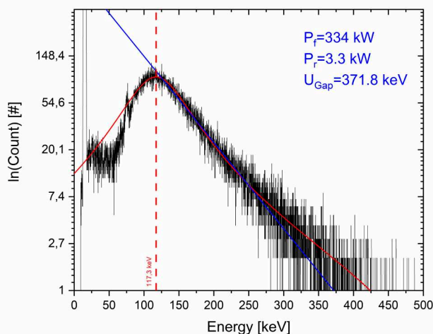
Figure 5: Gap voltage verification with X-ray energy measurement for the forward RF-power.
