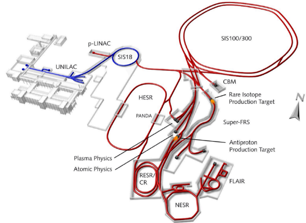
Figure 2: Schematic overview of the current GSI (blue) and the new FAIR complex in the complete expansion stage (red).
