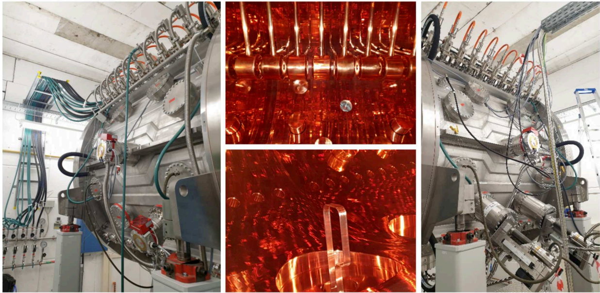
Figure 3: The copper plated FoS-Alvarez cavity section with a length of 1.9 m and 11 drift tubes. The drift tubes are installed at the top of the tank, but other combinations are possible. The bottom houses RF coupling and an service access. The new inductive incoupling loop for a 6 1/8" rigid RF-line is connected to the 1.8 MW RF-power amplifier. Three vacuum pumps and two dynamic plungers are installed at the FoS cavity.
