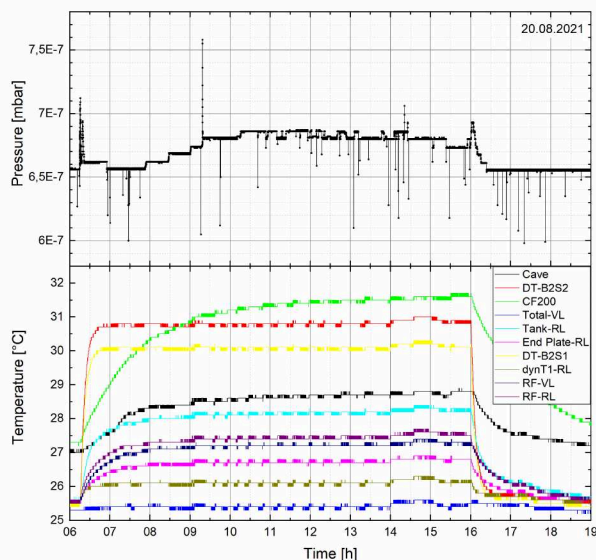
Figure 4: Measured vacuum pressure (top) and temperature (bottom) for constant RF-operation of the FoS-Alvarez at P_f=333 kW, P_r=3.3 kW.
