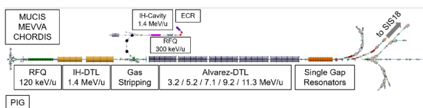
Figure 1: Schematic overview of the upgraded GSI UNILAC with five individual Alvarez-type post-stripper DTLs.
