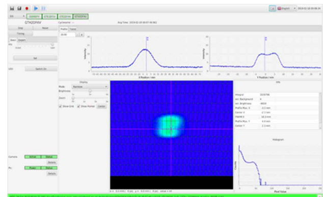
Figure 7: Screenshot of a beam spot on a scintillating screen with data evaluation like projections, FWHM, center of mass etc.
