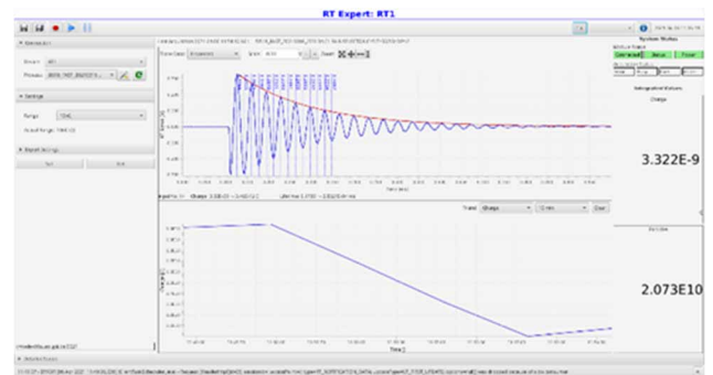
Figure 5: Typical resonant intensity signal using a resonant transformer with fast extracted ion beam.
