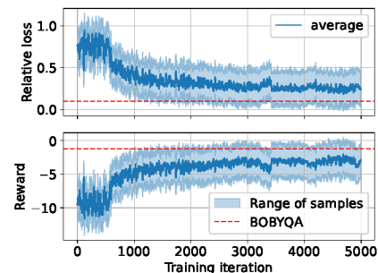
Figure 5: Training with Soft Actor Critic (SAC). The red line indicates the best result with the BOBYQA algorithms.
