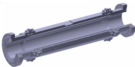
Figure 11: 3D model of the HEL BPM prototype.
