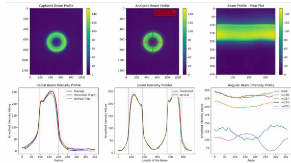
Figure 6: Transverse profile of a 4 keV, 25 mA, 25 \mu s long hollow electron beam as measured with a YAG:Ce screen.
