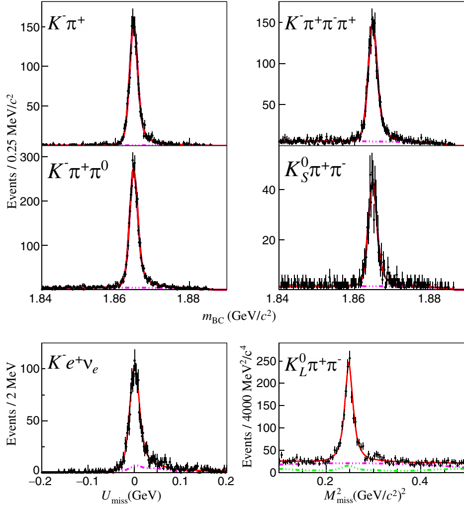
FIG. 3. Distributions and fits used to determine the DT yields for four fully reconstructed tags, and for the partially reconstructed tags K^- e^+ \nu_e and K_L^0 \pi^+ \pi^- . These distributions are of m_{BC} in the fully reconstructed case, and of U_{\text{miss}} ( M_{\text{miss}}^2 ) for the K^- e^+ \nu_e ( K_L^0 \pi^+ \pi^- ) case. In each plot the black dots with error bars are data, the total fit result is shown as the red solid line, the combinatorial background is shown as the pink dot-dashed line, and the sum of the combinatorial and the peaking background for the D \rightarrow K^- e^+ \nu_e and K_L^0 \pi^+ \pi^- DTs is shown as the green dashed line.
