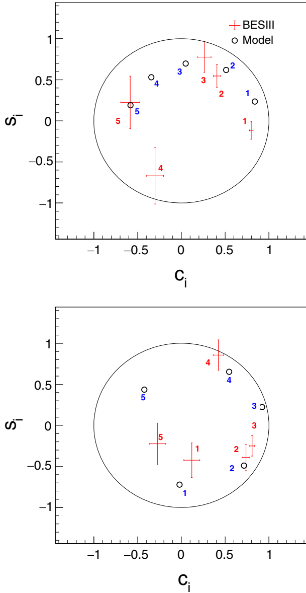
FIG. 5. Results of the c_i , s_i measurements for the equal- \Delta\delta_p -binning scheme (top) and the optimal-binning scheme (bottom). Also shown are the predictions based on the model from Ref. [17].
