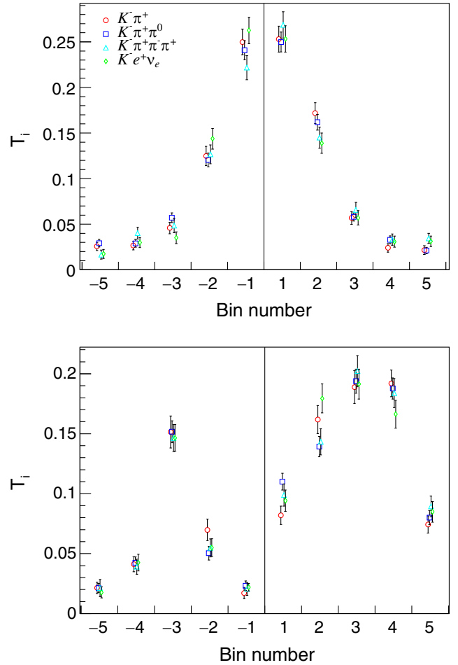
FIG. 4. Comparison of T_i between different flavor-tag modes. The top plot shows the equal- \Delta\delta_p binning and the bottom one the optimal binning.
