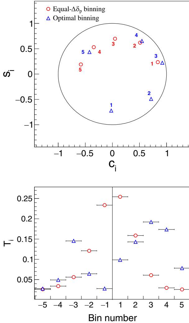
FIG. 1. Model predictions of c_i , s_i (top) and T_i (bottom) for the two binning schemes.
