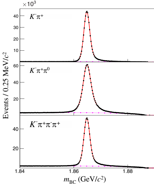
FIG. 2. Distributions and fits in m_{\text{BC}} used to determine the ST yields for the hadronic flavor-tag channels. The black dots with error bars are data, the total fit result is shown as the red solid line and the combinatorial background is shown as the pink dashed line.
