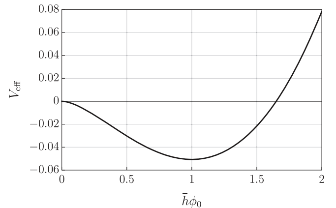
FIG. 2. Renormalized effective potential of the \gamma_{11} model for N_f = 1 and d_\gamma = 32 . The position of the minimum has been set to 1, namely \bar{h}v = 1 , in units of the square of an arbitrary dimensionful scale. The presence of a minimum at \phi_0 = v indicates the formation of a mass gap in the fermionic spectrum.
