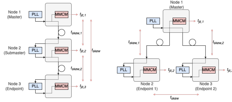
Figure 2. Clock distribution configurations for model validation: serial (left) and parallel (right).
