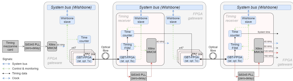
Figure 1. Architecture of the clock distribution chain in CBM.
