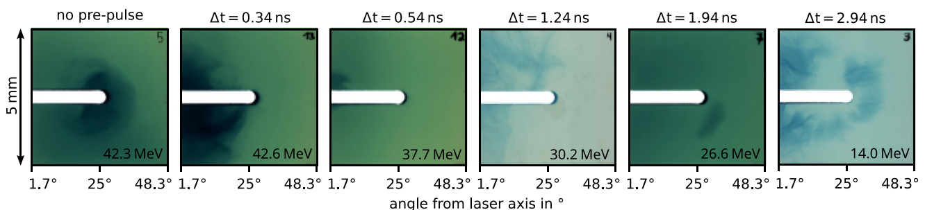
FIG. 7. RCFs of the last layer for each shot, corresponding to the highest measured proton energy. The RCF stack was positioned parallel to the target surface. Thus, the left side corresponds to an emission angle of 1.7^\circ , the center to 25^\circ (target normal), and the right side to 48.3^\circ relative to the laser propagation axis.
