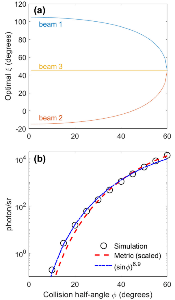
FIG. 4. Effect of varying collision angle \phi in three-color family of solutions. (a) Optimum beam polarization angles used in calculating peak photon brightness. (b) Photon brightness along \vec{k}_4 with optimum polarization (points); amplitude of polarization metric, scaled to fit (red); best fit model (blue).
