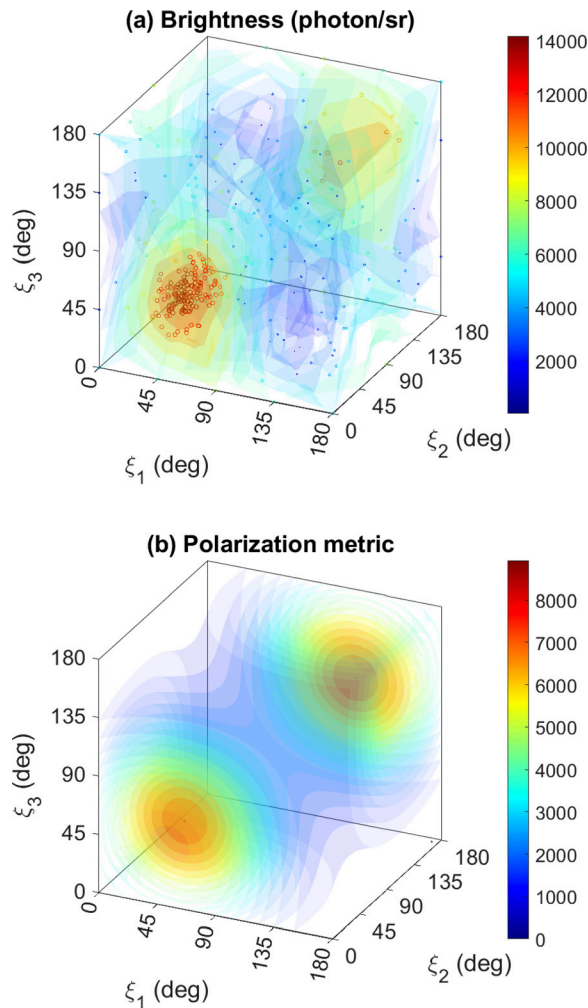
FIG. 3. Effect of polarization in the planar three-color geometry. (a) Brightness of scattered photons calculated along \vec{k}_4 for 318 simulations (points); interpolation over points (surfaces). (b) Evaluation of polarization metric for this case, Eq. (16).
