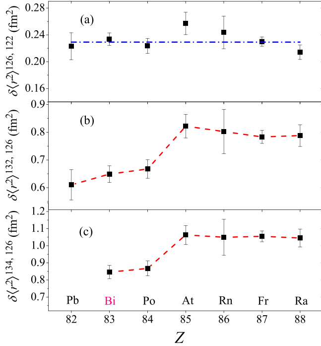
FIG. 5. Isotonic dependence of (a) \delta\langle r^2 \rangle^{126,122} , (b) \delta\langle r^2 \rangle^{132,126} , and (c) \delta\langle r^2 \rangle^{134,126} . The radon ( Z = 86 ) data from Refs. [15,18] were recalculated with the atomic factor scaled in accordance with its typical overestimation by the semiempirical method used in Ref. [15] (see details in Appendix B). Other experimental data are from the same sources as in Fig. 4. In panel (a), the dot-dashed line represents the weighted mean of the \delta\langle r^2 \rangle^{126,122} values. In panels (b) and (c), the dashed lines connect the data points to guide the eyes.
