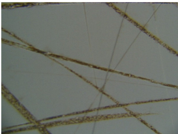
Fig. 43 Optical image (20x) of graphene (thick) and h-BN (thick) nanostripes on Si/SiO 2 wafer at applied pressure of \sim 200 Pa. The rubbings are performed manually. The number of rubbing circular cycles is 1000 for 200 ng bulk h-BN powder with 184 nm (commercial quality) crystallite size and 800 for graphite powder. Figure adapted from [250]
