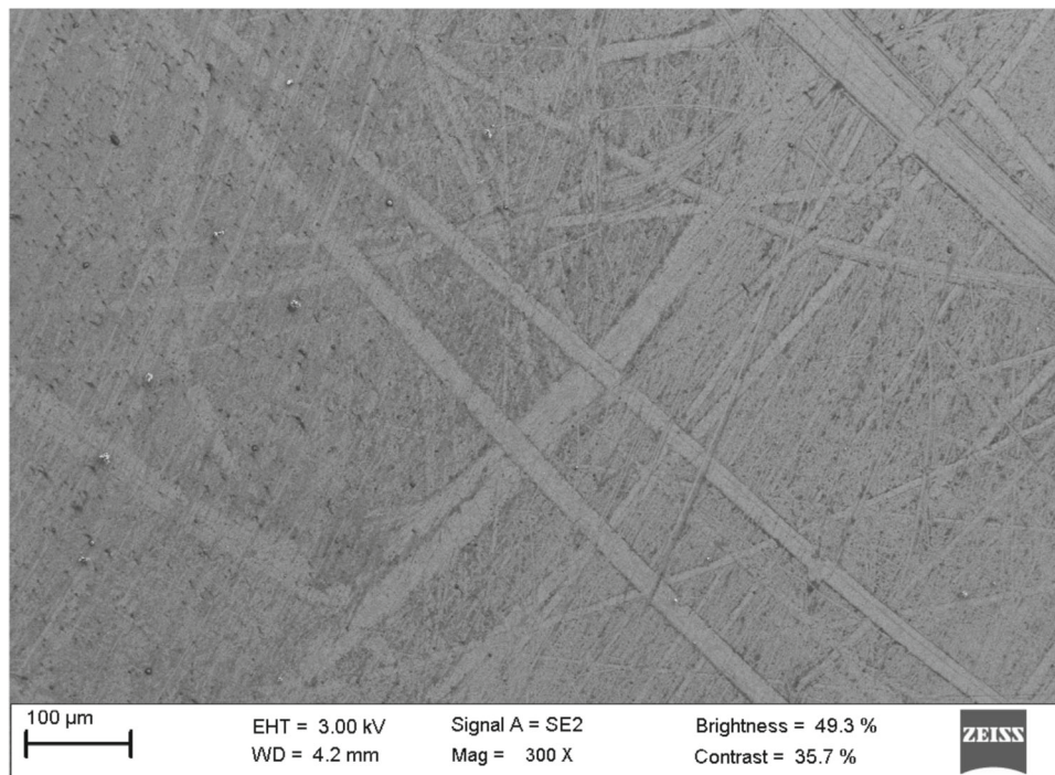
Fig. 42 Scanning electron microscope (SEM) image of mono- and few-layer graphene sheet consisting of the nanostripes on Si/SiO 2 substrate with atomically flat surface achieved using pressure of \sim 200 Pa at rubbing (with bulk graphite powder) circular cycles of 500. The rubbings are performed manually. Figure adapted from [250]
