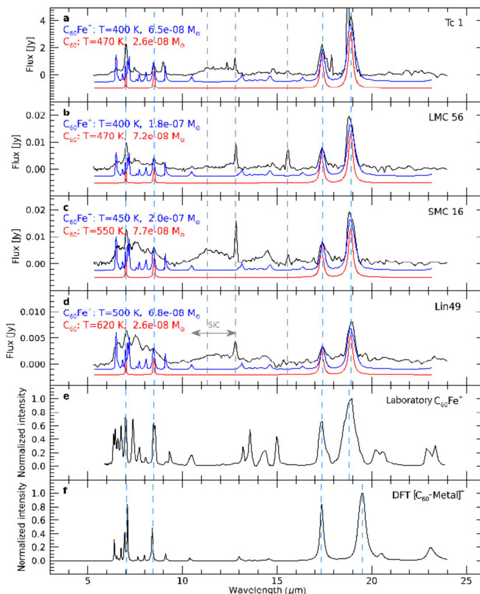
Fig. 11 Comparison between the Spitzer infrared spectra of four fullerene-rich PNe (black) and the thermal emission model for C_{60} (red) and C_{60}Fe^+ (blue). a Tc 1, b LMC 56, c SMC 16, d Lin49, e Laboratory infrared spectrum of C_{60}Fe^+ , and f Summed theoretical spectrum of [C_{60}-Metal]^+ . Figure reproduced from Ref [92]
