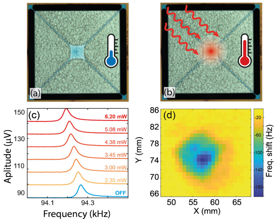
Fig. 20 Working principle of TMBs. A resonator at a certain temperature (a) has a specific resonant frequency of its mechanical modes (c - fundamental mode, OFF). Radiation absorbed by the device raises its temperature (b), simultaneously shifting its resonant frequency (c - increasing power). c—Typical mechanical resonator shift as a function of a 550 THz laser impinging power. d—Beam profiling of the 140 GHz source taken by scanning the position of a single TMB
