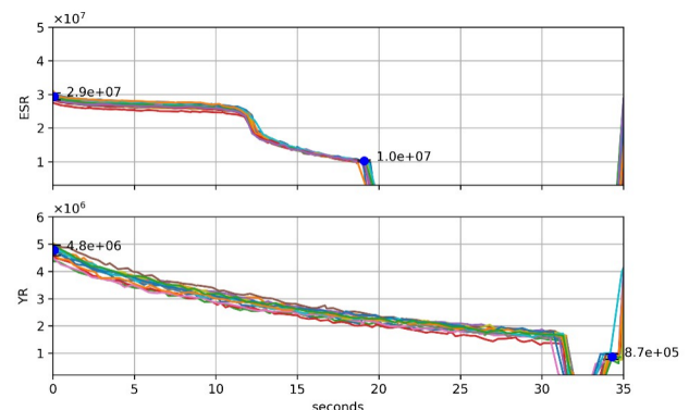
Figure 2: Transfer efficiency ESR – CRYRING@ESR (labelled with “YR”) measured to 39(1)%. In the upper graph, the number of particles stored in the ESR are plotted for a number of cycles. The second plot shows the number of particles stored for the corresponding cycle in CRYRING@ESR. The dots with error bars give the number of particles averaged over the analyzed 14 cycles.
