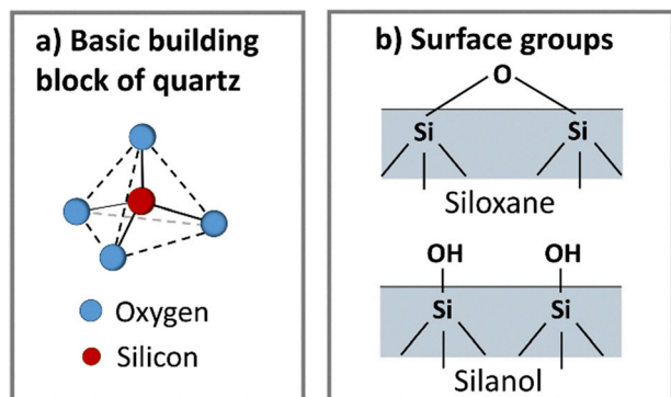
Fig. 5 Basic building block of quartz (panel (a)) and functional groups on the quartz surface (panel (b)).
