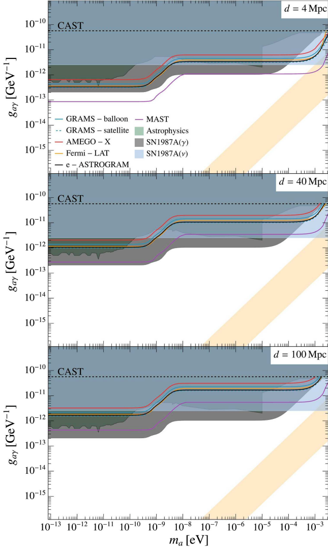
FIG. 6. Sensitivities of e-ASTROGRAM [88], AMEGO-X [89], Fermi -LAT [90], GRAMS-balloon [91], GRAMS-satellite [91], and MAST [92] in the plane g_{a\gamma} vs m_a assuming that g_{a\mu} and g_{a\gamma} are related as in Eq. (11). We assume a BNS system at the same sky location as the GW170817 event, at a distance of d = 4 Mpc (upper panel), d = 40 Mpc (middle panel), and d = 100 Mpc (lower panel) from the observer, respectively. The gray bound represents the limit for the SN 1987A derived using the spectra shown in Fig. 3 and taking into account the conversion probability in the progenitor and in the Milky Way magnetic fields [32,33], and the dashed line the most recent CAST bound from solar axions [95]. Finally, the bounds in green correspond to constraints from other astrophysical observations [96–99]. We highlight that bounds in green are derived by assuming ALPs coupled to photons only. We refer the reader to Table II.
