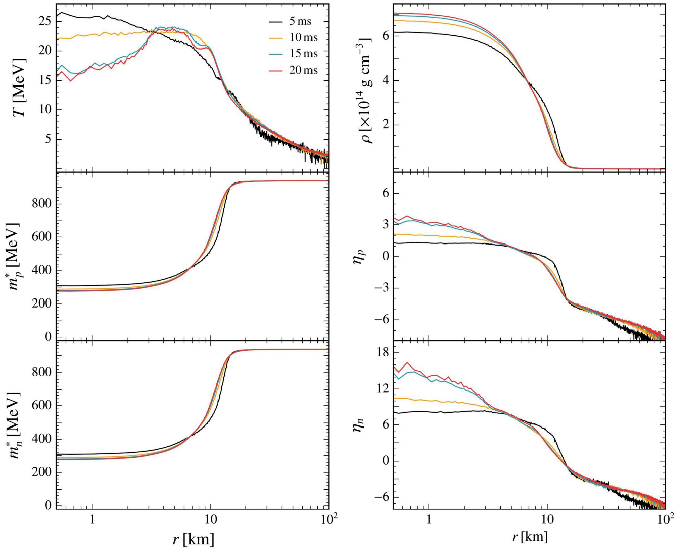
FIG. 1. Radial evolution at different postmerging times for different quantities from the adopted BNS merger model. Left panels: temperature T (top), effective proton mass m_p^* (middle), and effective neutron mass m_n^* (bottom). Right panels: density \rho (top), proton degeneracy factor \eta_p (middle), and neutron degeneracy factor \eta_n (bottom).
