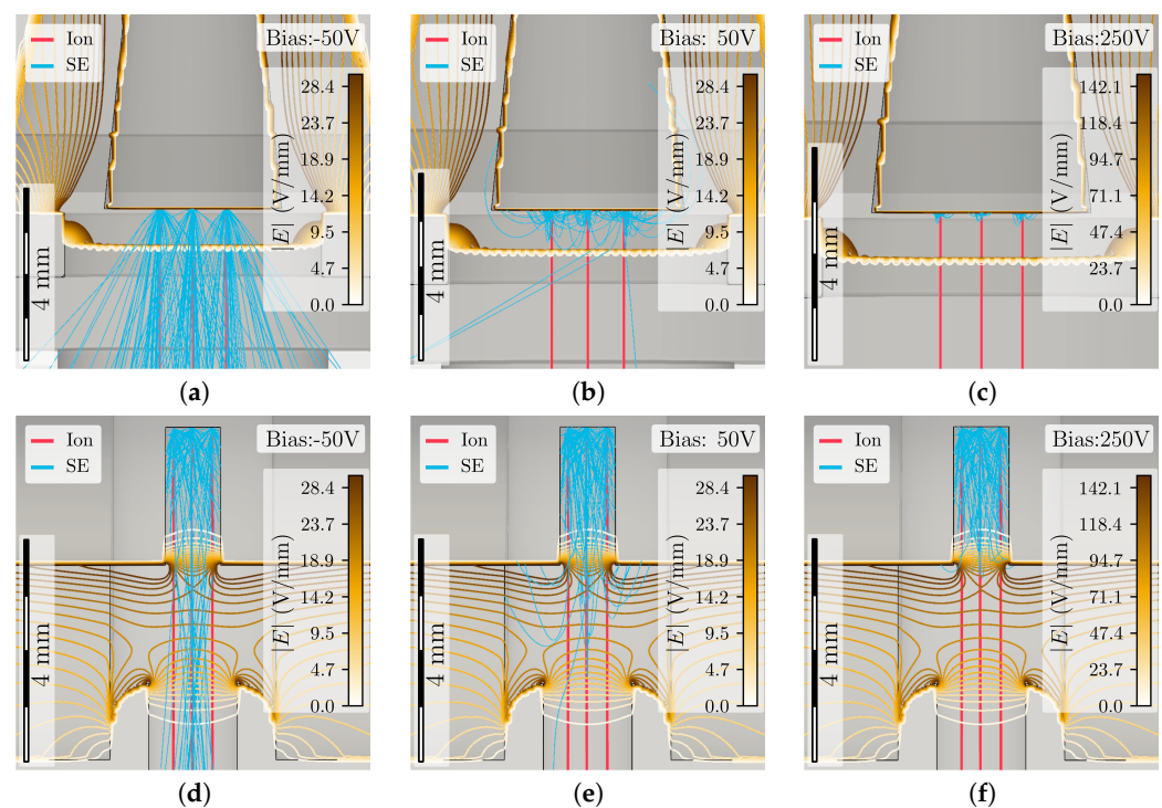
Figure 3. CST PT simulations of the ACFFC (top) and radially coupled Fast Faraday Cup (RCFFC) (bottom) for the bias settings -50 V (a,d), 50 V (b,e) and 250 V (c,f). The incoming ions are shown in red and the emitted SEs are blue. The equipotential lines of the bias field are overlaid to the actual geometry of the FFCs close to the collector surfaces.
