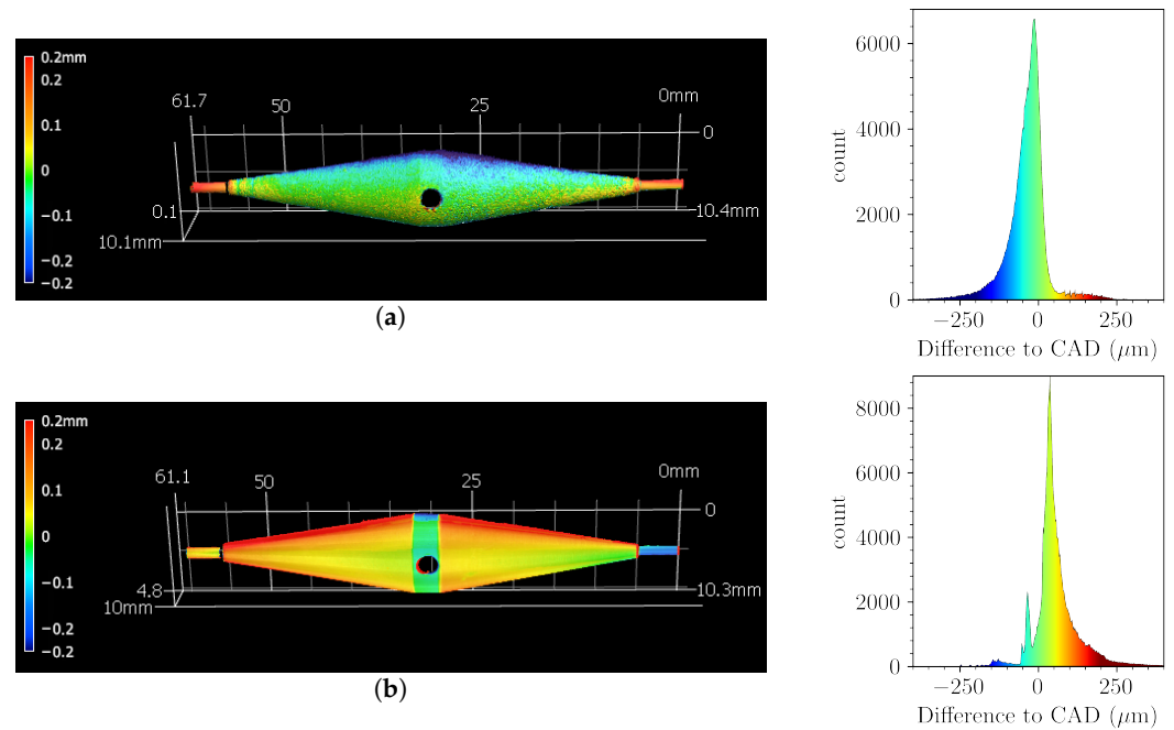
Figure 14. Three-dimensional scan of the difference to the CAD model for the AM (a) and the CM (b) version of the collector. On the right-hand side, the corresponding histograms display the distribution of these differences in terms of count of measurements, using the same color coding as the 3D scans.
