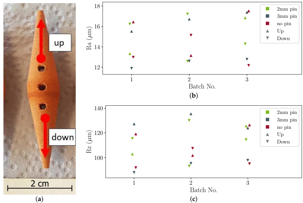
Figure 11. (a) Measurement of the surface roughness starting from two points with a probe diameter of 5\ \mu\text{m} on a length of 8 mm upwards and downwards, (b) shows the measured average profile height deviations from the mean line R_a , and (c) the maximum peak height to valley height R_z .
