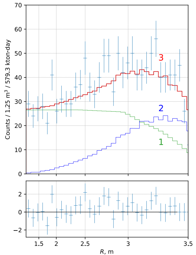
Fig. 6 The fitted Borexino radial spectrum. The curve 1 corresponds to the uniform part of the spectrum whilst the curve 2 is the radial distribution of the simulated external background events. The decline in the distribution of uniform events is caused by the fiducial volume non-sphericity. The fit (curve 3) is complementary to the energy fit on Fig. 5
