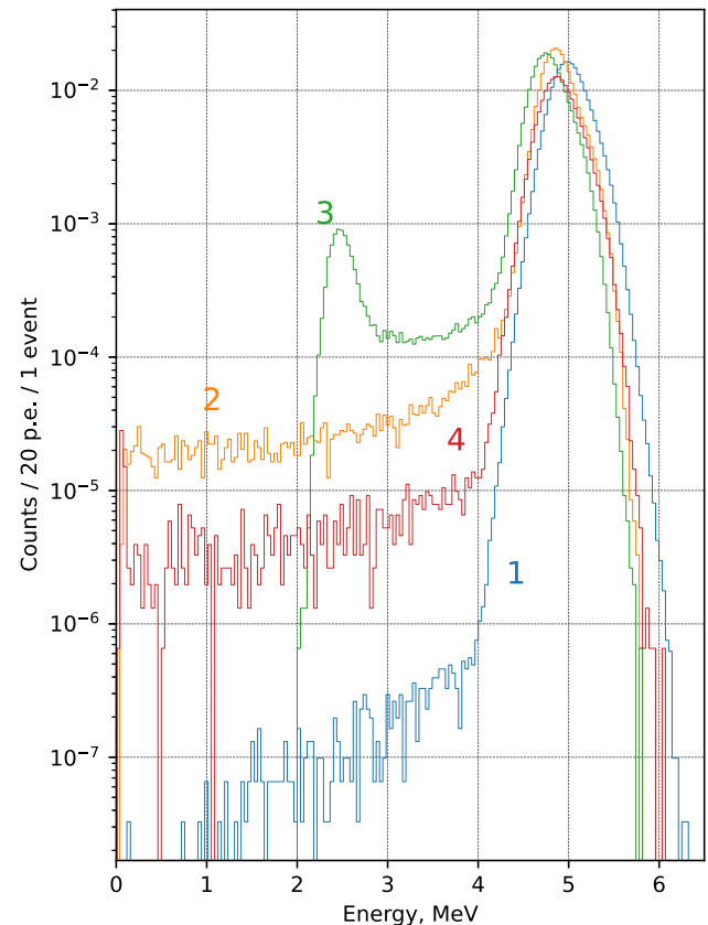
Fig. 3 Simulated responses to axion interactions in the Borexino IV: 1 - axioelectric effect (5.49 MeV electrons), 2 - Compton axion to photon conversion (electrons and \gamma -quanta), 3 - decay A \rightarrow 2\gamma , 4 - Primakoff conversion (5.49 MeV \gamma -quanta). The response functions are normalized to single axion interaction for decay in 5 m radius sphere
