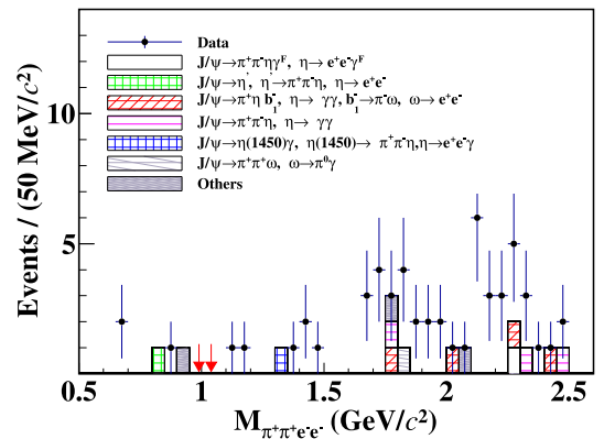
Fig. 3. (color online) The distribution of M_{\pi^+ \pi^+ e^- e^-} for events in the range of M_{\gamma \gamma} \in (0.52, 0.57) GeV/ c^2 , where the points with error bars are data, the histogram in different styles represent different sources of background modes shown in the legends. The red arrows show the signal region.
