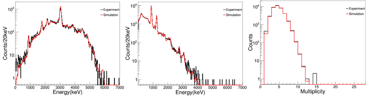
Fig. 8. The total absorption spectrum, sum-of-segments, and multiplicity in ^{70}\text{Zn} resulting from the ground-state decays of ^{70}\text{Cu} .
