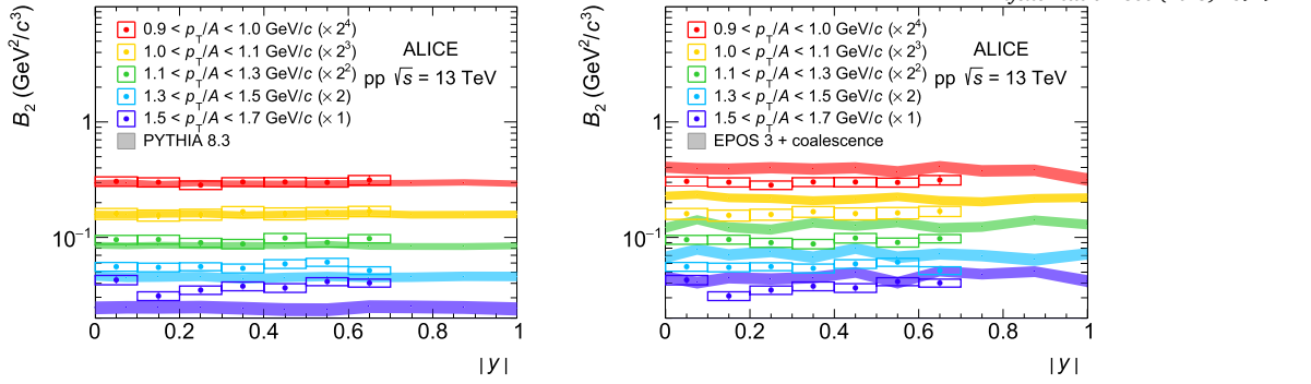
Fig. 4. Coalescence parameter B_2 as a function of rapidity, for fixed transverse momentum per nucleon values. Statistical and systematic uncertainties on the data points are represented by vertical bars and boxes, respectively. The statistical uncertainties are smaller than the size of the markers in the reported scale and, hence, not visible. Bands show the model predictions from PYTHIA 8.3 (left panel) and from a coalescence model [57] used as afterburner of EPOS 3 (right panel), the width reflecting the statistical uncertainties.
