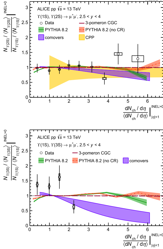
Fig. 4. Top: Excited-to-ground state self-normalized yield ratio ( \Upsilon(2S) over \Upsilon(1S) ) as a function of self-normalized charged-particle multiplicity, compared to model predictions from 3-pomeron CGC approach [67], PYTHIA 8.2 [5], comovers [39,44], and CPP [65] calculations. Bottom: Excited-to-ground state self-normalized yield ratio ( \Upsilon(3S) over \Upsilon(1S) ) as a function of self-normalized charged-particle multiplicity, compared to PYTHIA 8.2 and comovers predictions. The vertical error bars represent the statistical uncertainty, while the systematic uncertainties are depicted as boxes.
