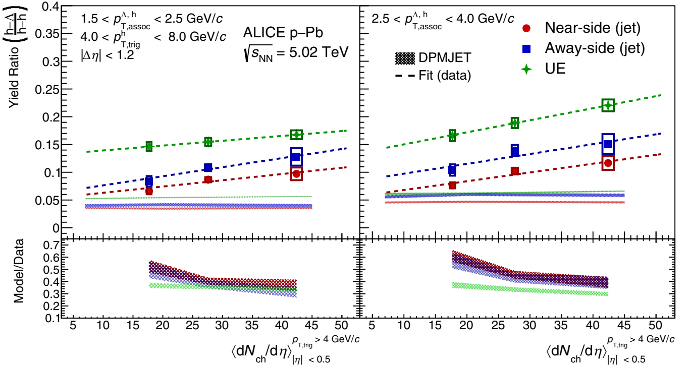
FIG. 6. The per-trigger pairwise yield ratios R_i^{\Delta/h} \equiv Y_i^{\Delta/h}/Y_i^{h-h} ( i = near side, away side, UE) as a function of multiplicity in the lower (left) and higher (right) associated momentum ranges. The statistical (systematic) uncertainties are shown as vertical lines (boxes). Linear fits to the data are given as dashed lines. The ratios predicted by DPMJET are presented as shaded bands, with the width of the band representing the uncertainty of the model. The ratios of the model to the data are also shown as shaded bands in the bottom panels, where the width of the band represents the uncertainty of the ratio.
