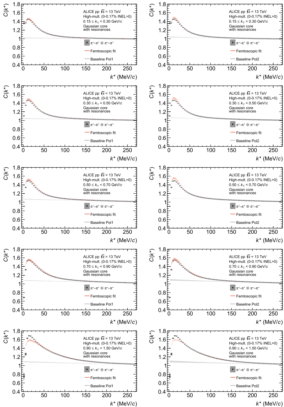
Fig. 10 Correlation functions of \pi - \pi in bins of k_T for HM collisions, the fits on the left (right) are performed using CATS [31] employing the RSM and assuming a polynomial of first (second) degree as back-
