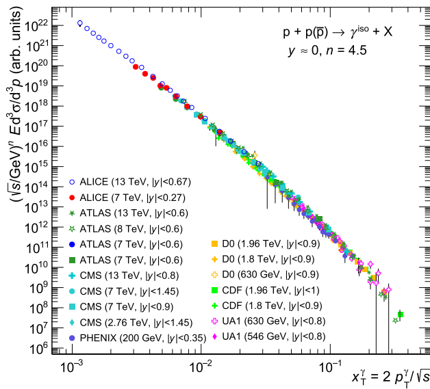
Fig. 9 ALICE data compared to previous measurements of isolated-photon spectra in pp and p \bar{p} collisions as a function of x_T^\gamma where the invariant cross sections have been scaled by (\sqrt{s})^n with n = 4.5 (taken from Ref. [2]). For this comparison, only the results covering midrapidity are shown
