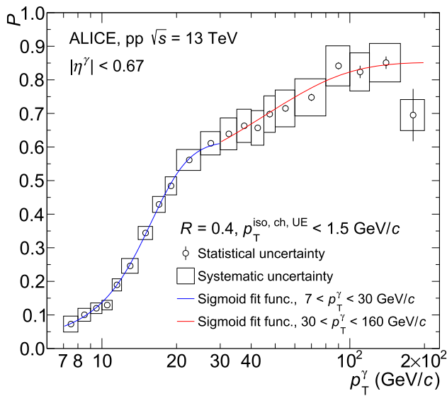
Fig. 2 Purity of the isolated-photon sample as a function of p_T^\gamma calculated using Eq. (8). The statistical and systematic uncertainties have been evaluated as discussed in Sect. 4. The red and blue lines are the results of a fit to the measured purity using a two-sigmoid-function described by Eq. (11) for two different transverse momentum intervals
