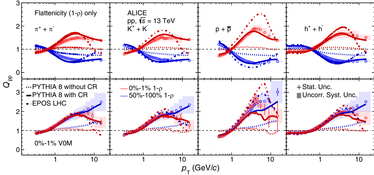
FIG. 5. The Q_{pp} ratio of \pi , K , p , and h^\pm for the 0%–1% and 50%–100% 1-\rho classes (top row) and for the same 1-\rho classes in HM (0%–1% VOM class) events (bottom row). The data are compared with PYTHIA 8 and EPOS LHC model predictions. The statistical and systematic uncertainties are represented with bars and shaded areas.
