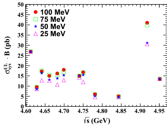
FIG. 5. The upper limits of the product of the cross section and branching fraction \sigma(e^+e^- \rightarrow \gamma X) \cdot B(X \rightarrow D_s^+ D_{s1}^-(2536) + \text{c.c.}) at each energy points assuming the width \Gamma_X = 25, 50, 75 , or 100 MeV at 90% CL.
