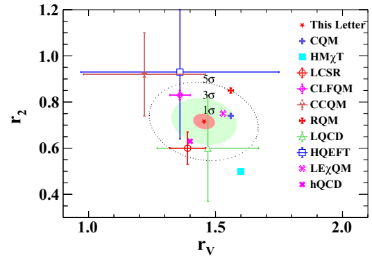
FIG. 4. Comparisons of the measured r_V and r_2 in this Letter with various theoretical calculations [16–28]. The correlation coefficient between the measured r_V and r_2 is -0.17 .
