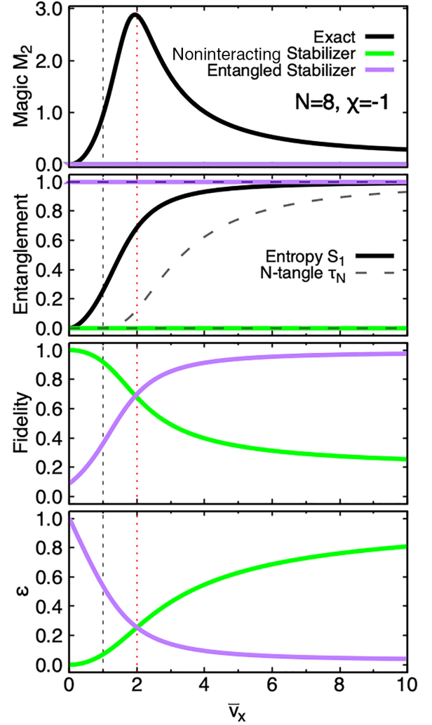
FIG. 2. From bottom to top panel: relative energy difference \varepsilon , fidelity, entanglement, and stabilizer 2-Rényi entropy \mathcal{M}_2 , in a system with N = 8 spins, as a function of the interaction strength \bar{v}_x . The exact solution is shown with black curves, the unentangled (noninteracting) stabilizer state |\Psi_{s,1}\rangle^{(N)} = |1\rangle^{\otimes N} is shown with green curves and the entangled stabilizer state |\Psi_{s,2}\rangle^{(N)} is shown with purple curves. In the entanglement panel, the von Neumann entropy is displayed with plain lines while the N -tangle \tau_N is shown with dashed lines. The black dashed vertical line denotes the critical point between normal (spherical) and parity-broken (deformed) phases, while the red dotted vertical line denotes the transition from unentangled to entangled stabilizer ground state.
