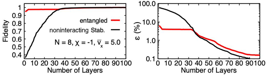
FIG. 10. ADAPT-VQE convergence for a system with N = 8 spins, \chi = -1 , and \bar{v}_x = 5 . The left and right panel show the fidelity and relative energy error of the ADAPT-VQE wave function, receptively. The black curve shows the results obtained with the unentangled reference state |\phi\rangle = |\Psi_{s,1}\rangle , while the red curve shows the results for |\phi\rangle = |\Psi_{s,2}\rangle .
