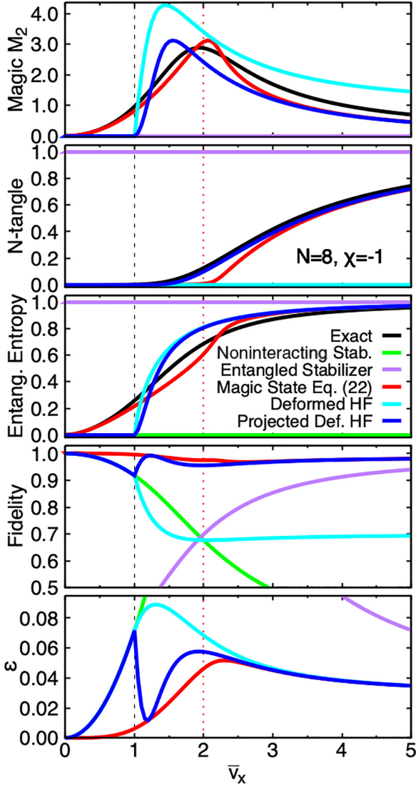
FIG. 4. Relative energy difference \epsilon , fidelity, von Neumann entanglement entropy S_1^{(N)} , N -tangle \tau_N , and SRE \mathcal{M}_2 in a system with N = 8 spins and \chi = -1 . The exact solution appears in black. The unentangled and entangled stabilizer states, |\Psi_{s,1}\rangle^{(N)} and |\Psi_{s,2}\rangle^{(N)} , are shown in green and purple curves, respectively. The state obtained via Eq. (22) is shown with red curves. For comparison, the deformed HF without and with projection are shown with cyan and blue curves, respectively.
