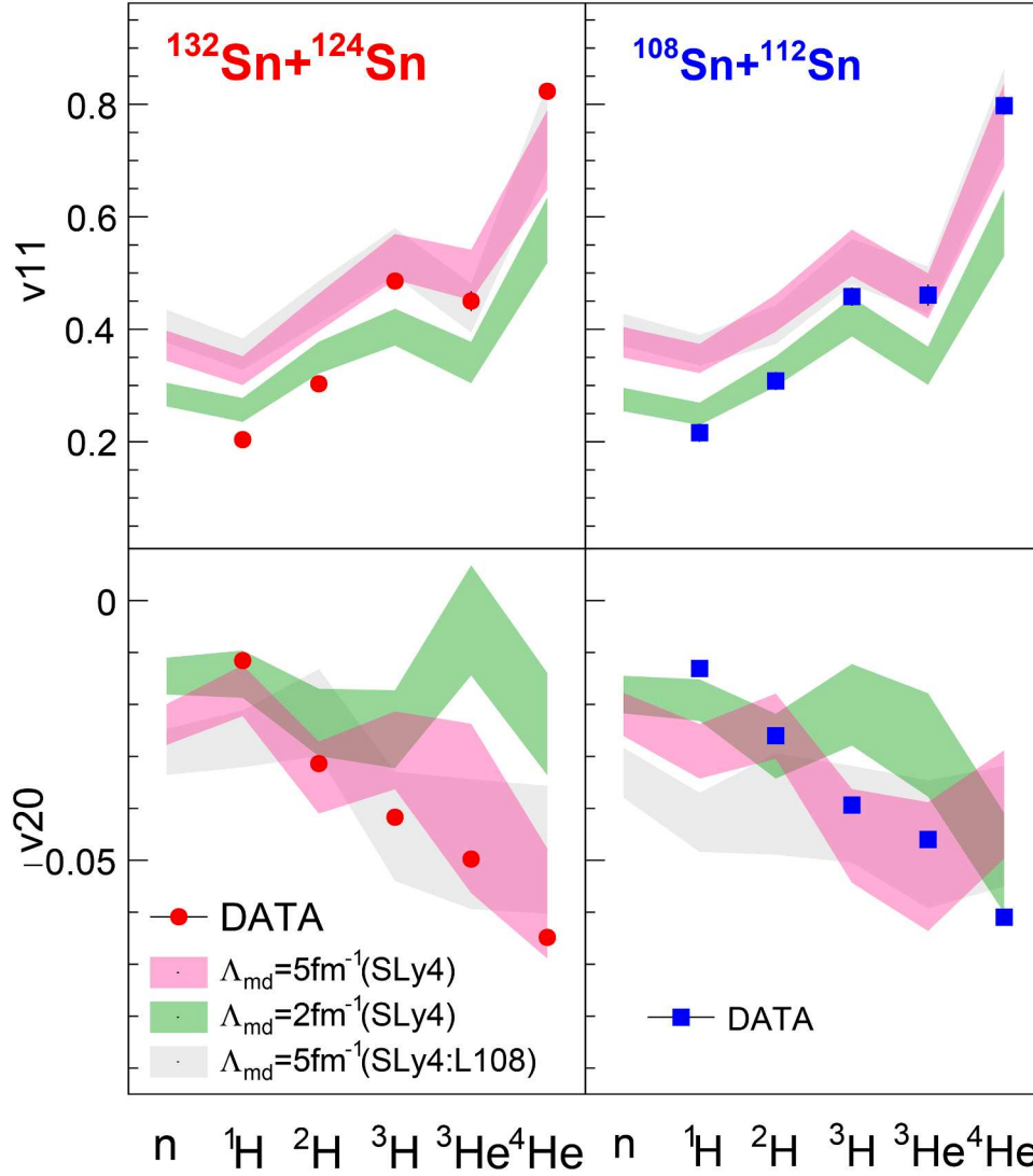
Fig. 5. Particle dependence of v_{11} , v_{20} , plotted on top and bottom, respectively. Left and right columns correspond to ^{132}\text{Sn} + ^{124}\text{Sn} and ^{108}\text{Sn} + ^{112}\text{Sn} , respectively. AMD calculations with \Lambda_{\text{md}} = 2 \text{ fm}^{-1} (SLy4) (green band), \Lambda_{\text{md}} = 5 \text{ fm}^{-1} (SLy4) (magenta band), and \Lambda_{\text{md}} = 5 \text{ fm}^{-1} (SLy4 : L108) (gray band) are also plotted for comparison. (For interpretation of the references to colour in this figure legend, the reader is referred to the web version of this article.)
