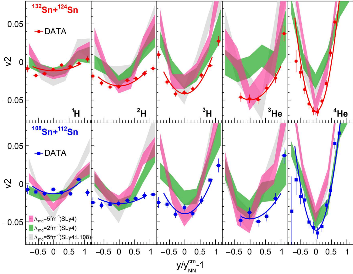
Fig. 6. The elliptic flow, v_2 plotted as a function of scaled rapidity. Top and bottom panels are for ^{132}\text{Sn} + ^{124}\text{Sn} and ^{108}\text{Sn} + ^{112}\text{Sn} , respectively. Solid lines in the figure show relevant results with a parabolic function, and the minimum v_2 is determined as v_{20} . AMD calculations with \Lambda_{\text{md}} = 2 \text{ fm}^{-1}(\text{SLy4}) (green band), \Lambda_{\text{md}} = 5 \text{ fm}^{-1}(\text{SLy4}) (magenta band), and \Lambda_{\text{md}} = 5 \text{ fm}^{-1}(\text{SLy4:L108}) (gray band) are also plotted for comparison. (For interpretation of the references to colour in this figure legend, the reader is referred to the web version of this article.)
