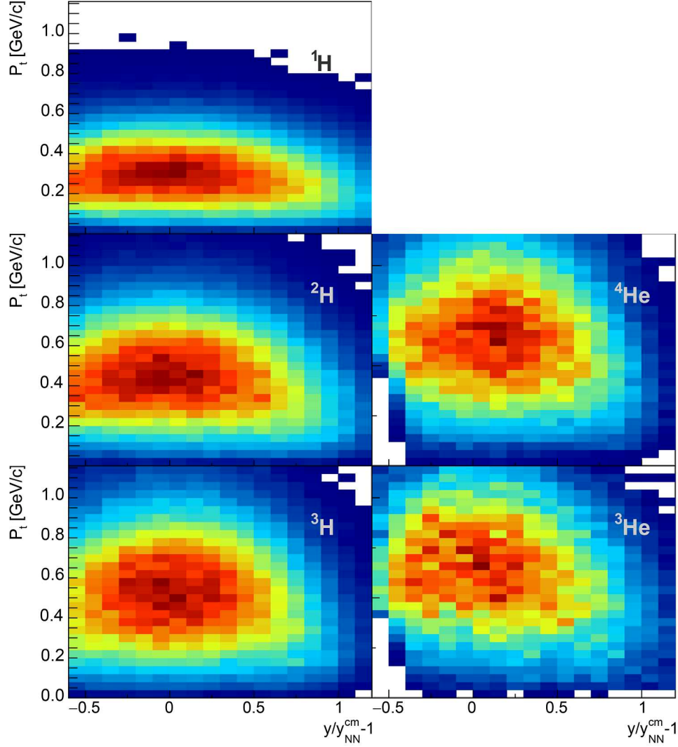
Fig. 1. The S \pi RIT-TPC acceptance for light charged particles for the scaled impact parameter within 0 \leq b_0 \leq 0.15 . The horizontal axis is the scaled rapidity, y/y_{NN}^{cm} - 1 , where y is the rapidity of the detected particle in the laboratory frame and the y_{NN}^{cm} is the rapidity of the nucleon-nucleon ( NN ) center-of-mass in the laboratory frame. The vertical axis corresponds to the transverse momentum. To minimize contamination from triton on {}^3\text{He} , y/y_{NN}^{cm} - 1 > -0.3 was analyzed, while y/y_{NN}^{cm} - 1 > -0.5 for other particles.
