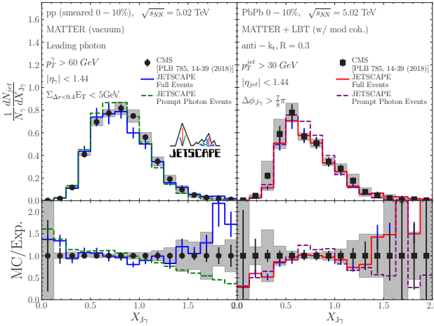
Figure 2. Photon-triggered jet asymmetry in p - p and 0 – 10% Pb - Pb collisions at \sqrt{s_{NN}} = 5.02 TeV, compared with CMS experimental results [3]. The solid and dashed lines represent total inclusive and prompt photon events, respectively. The bottom panel shows the ratio of JETSCAPE results to the experimental results.
