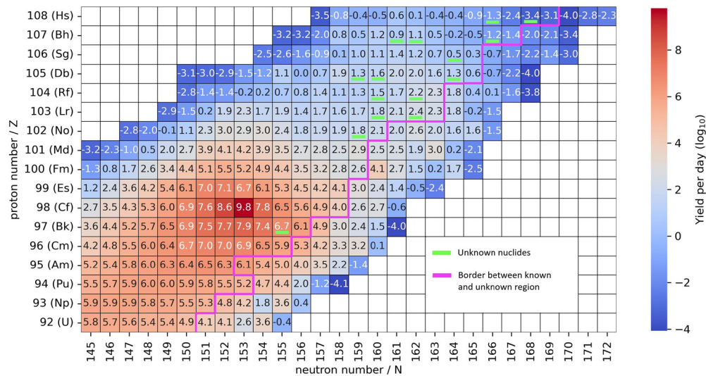
Fig. 7. The estimated yield per day at the velocity filters, based on cross-section calculations using Langevin-type dynamical model for the ^{48}\text{Ca} + ^{251}\text{Cf} reaction, at E_{\text{lab}} = 293 MeV, is presented. The following realistic values were considered: a ^{48}\text{Ca} beam intensity ( I_{\text{beam}} ) of 1.2 \mu\text{A} , a ^{251}\text{Cf} target thickness ( D_t ) of 500 \mu\text{g}/\text{cm}^2 , and an efficiency of 1% for an ideal experimental case with optimized field settings. The solid magenta line represents the boundary between the already discovered region of nuclides and the yet-to-be-discovered region. Within the discovered region, 15 nuclides, marked in green, are yet to be found and are situated between regions of nuclides discovered through cold and hot fusion reactions.
