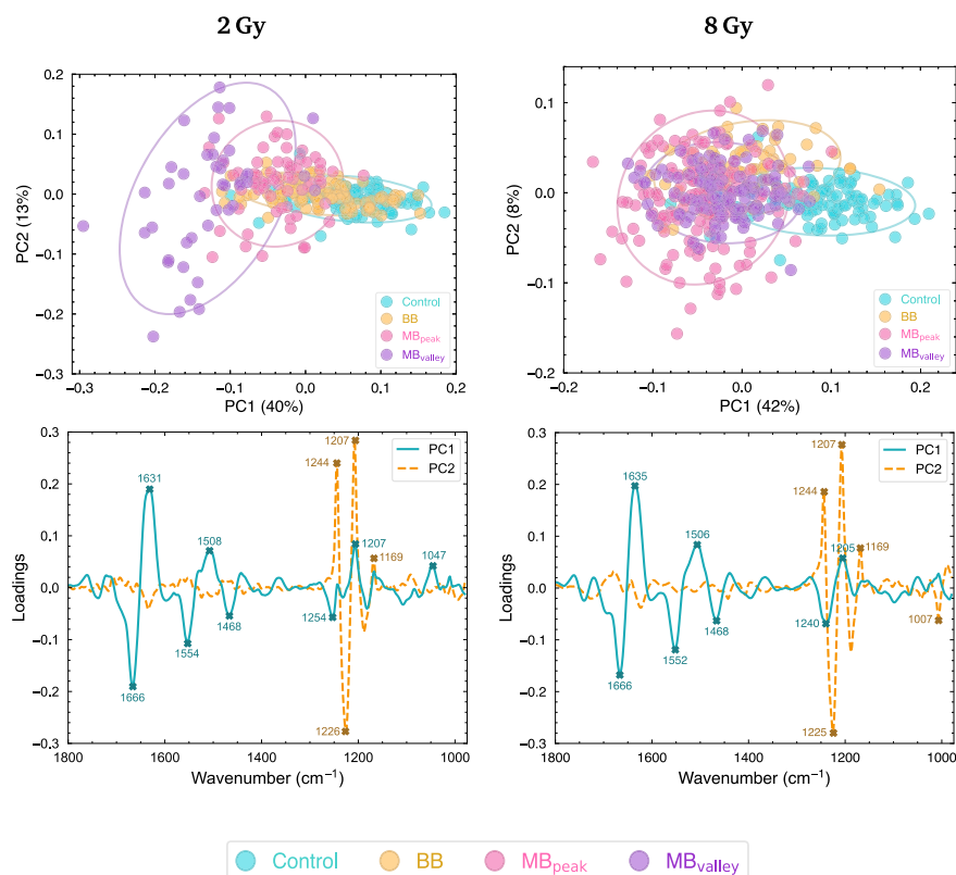
Fig. 4. PCA in the A+FP (1800–980 \text{cm}^{-1} ) spectral regions of LM8 mouse osteosarcoma cells irradiated with 2 Gy or 8 Gy carbon beams. For each spectral region, the PC scatter plots (upper row) and loadings (lower row) are included. Each point on the PC scatter plots represents a cell spectrum, and colours correspond to the irradiation configurations: blue for Control (non-irradiated), orange for BB, pink for \text{MB}_{\text{peak}} and purple for \text{MB}_{\text{valley}} . 95% confidence ellipses are included, and explained variances by the PCs are shown in parentheses. In the loadings, the contribution of each spectral band to data separation along PC1 is indicated by solid blue lines, while the bands contributing to the separation along PC2 are indicated by dashed orange lines. The most relevant IR peaks contributing to cluster delineation along PC1 or PC2 are marked with blue or orange labels and crosses, respectively. Indicated doses refer to the mean dose for both CBB and CMBRT modalities.
