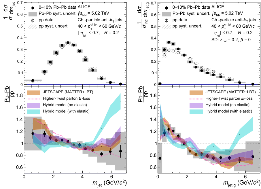
Fig. 1. ALICE measurements of ungroomed m_{\text{jet}} (left) and groomed m_{\text{jet,g}} (right) using R = 0.2 charged-particle jets with 40 < p_{\text{T}}^{\text{ch,jet}} < 60 GeV/c in pp and Pb-Pb collisions at \sqrt{s_{\text{NN}}} = 5.02 TeV compared to models. The bottom panel shows the ratio of Pb-Pb distributions to pp, which quantifies the substructure modifications from quenching.
