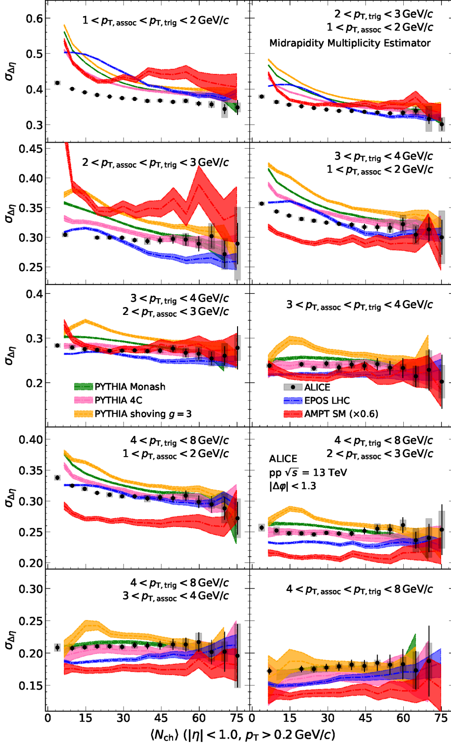
Figure 6. Multiplicity-dependence of near-side peak widths for all p_{T, \text{trig}} and p_{T, \text{assoc}} intervals measured in pp collisions at \sqrt{s} = 13 \text{ TeV} , compared with MC models. Multiplicities are estimated at midrapidity. The model results are shown as coloured bands with the width of the band denoting the statistical uncertainties. The error bars (boxes) represent the statistical (systematic) uncertainties in the experimental data. The AMPT calculations are scaled by a factor of 0.6 in all panels for visibility.
