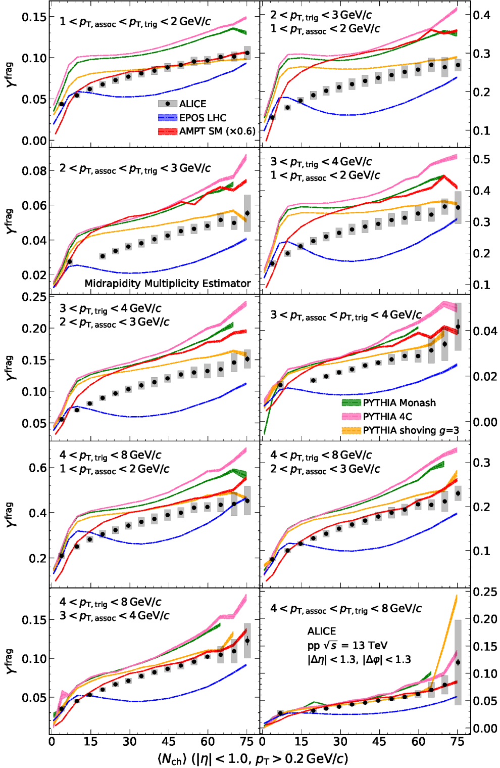
Figure 5. Multiplicity-dependence of near-side peak yields for all p_{T, \text{trig}} and p_{T, \text{assoc}} intervals measured in pp collisions at \sqrt{s} = 13 TeV, compared with MC models. Multiplicities are estimated at midrapidity. The model results are shown as coloured bands with the width of the band denoting the statistical uncertainties. The error bars (boxes) represent the statistical (systematic) uncertainties in the experimental data. The AMPT calculations are scaled by a factor of 0.6 in all panels for visibility.
