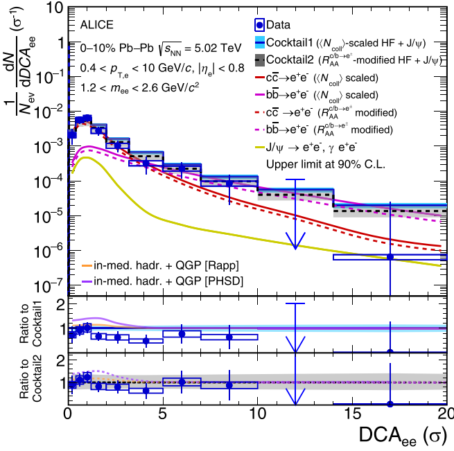
FIG. 13. Top panel: Inclusive e^+e^- yield in the 10% most central Pb–Pb collisions at \sqrt{s_{NN}} = 5.02 TeV as a function of DCA_{ee} in the mass range 1.2 < m_{ee} < 2.6 GeV/c 2 , compared with the expected e^+e^- contributions from known hadronic decays, including two different estimations for dielectrons from correlated heavy-flavor hadron decays (see text). Bottom panels: Ratios of data to cocktails, together with two predictions for thermal radiation from the medium [36,100]. Statistical and systematic uncertainties on the data are shown as vertical bars and boxes, respectively. The total uncertainty of the cocktails is represented as a band.
