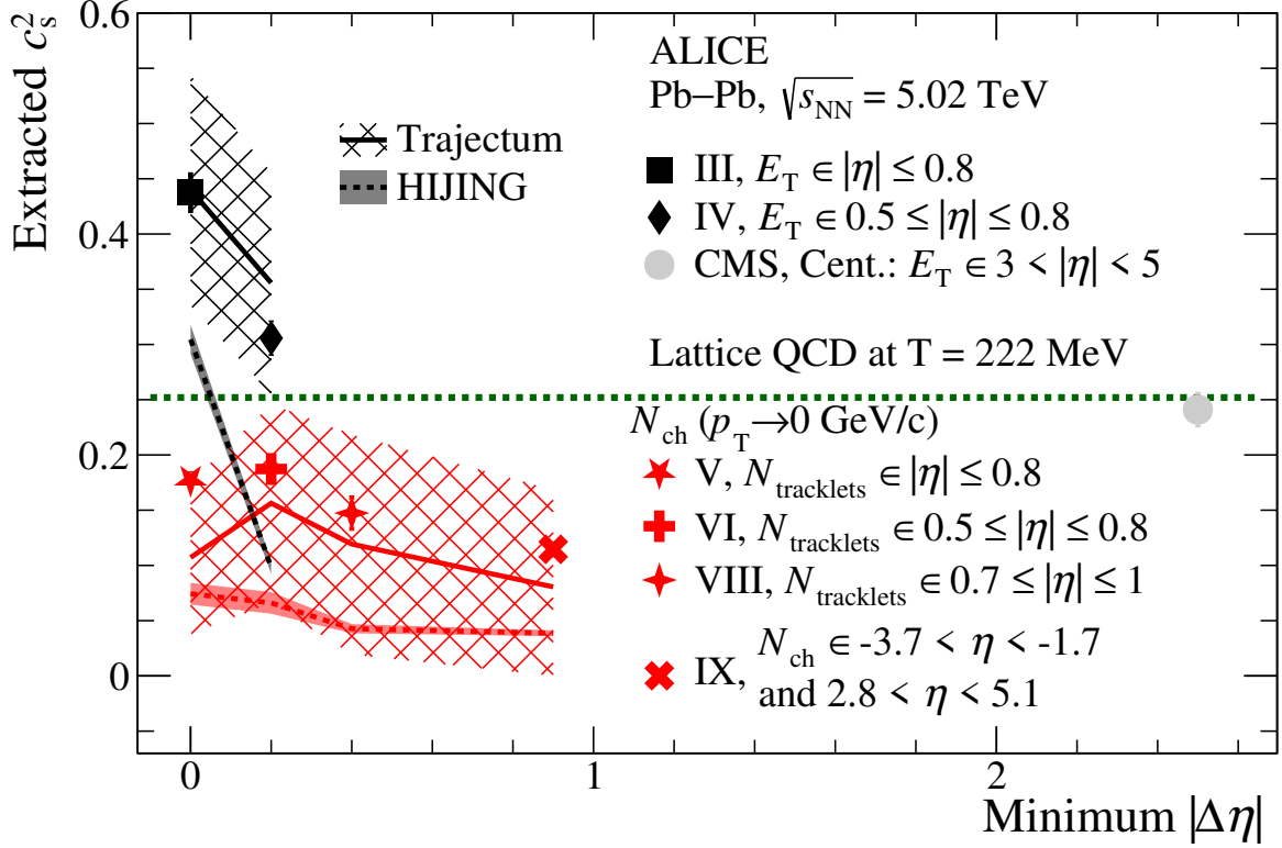
Figure 6. Extracted c_s^2 as a function of the minimum pseudorapidity gap between the centrality estimation and transverse-momentum spectra measurement in Pb-Pb collisions at \sqrt{s_{\text{NN}}} = 5.02 TeV. The results are compared with the c_s^2 value measured by the CMS collaboration (with a minimum |\Delta\eta| = 2.5 ) [21]. The uncertainty bars around the data points represent the sum in quadrature of the statistical and systematic uncertainties (not visible). Predictions from Trajectum [55–57] are shown as continuous lines, with mesh bands indicating the total uncertainty (statistical and systematic combined in quadrature). Predictions from the HIJING [42] model are shown as dashed lines, with shaded bands representing statistical uncertainty only. See the main text for details on the uncertainty estimation in the model c_s^2 values. The horizontal dashed green line indicates the Lattice QCD prediction of c_s^2 for deconfined matter, as calculated by the HotQCD collaboration [17]. Centrality-estimator definitions are presented in table 1.
