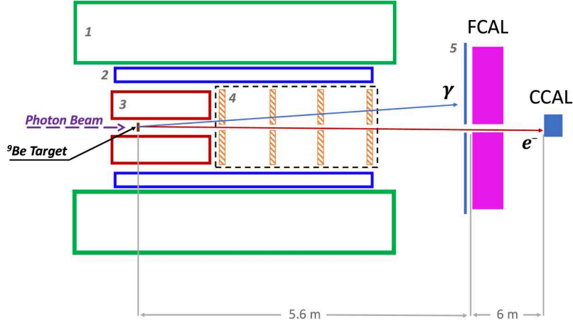
Fig. 2. Detector layout for the PrimEx- \eta experiment. Numbered components include (1) solenoid magnet, (2) barrel electromagnetic calorimeter, (3) central drift chamber, (4) forward drift chambers, and (5) time-of-flight wall. The scattered photons and electrons from Compton scattering events were detected by the Forward Calorimeter (FCAL) and the Compton Calorimeter (CCAL). Not drawn to scale.
