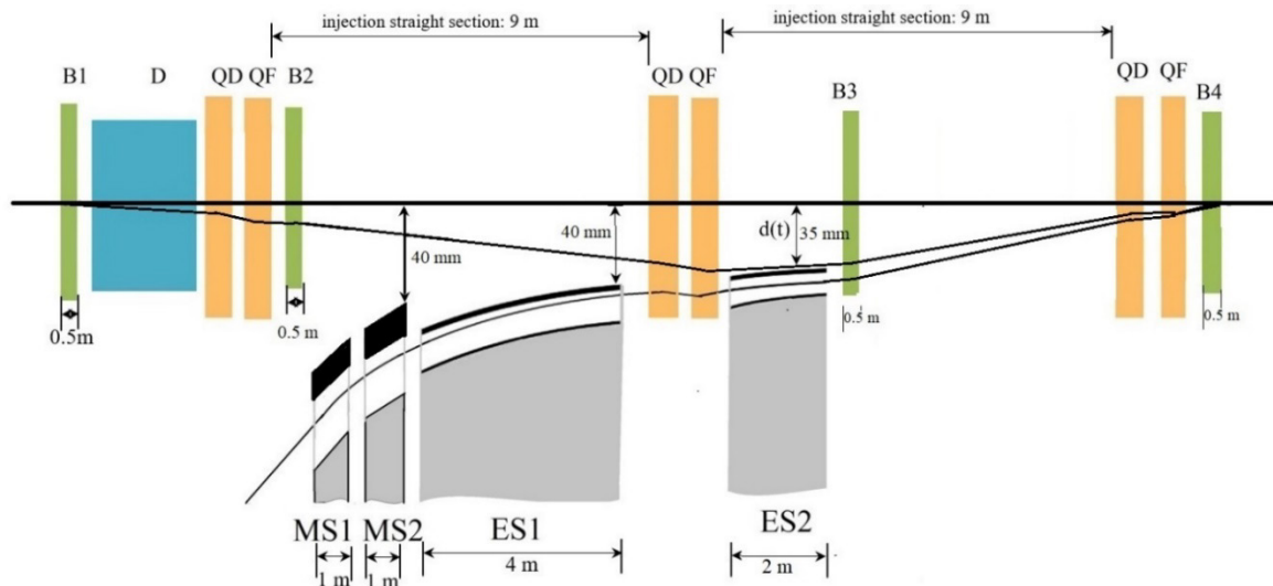
Figure 2: Proposed layout of the multi-turn injection system for SIS100, including two electrostatic septa (ES1, ES2) and bumper magnets (B1–B4).
