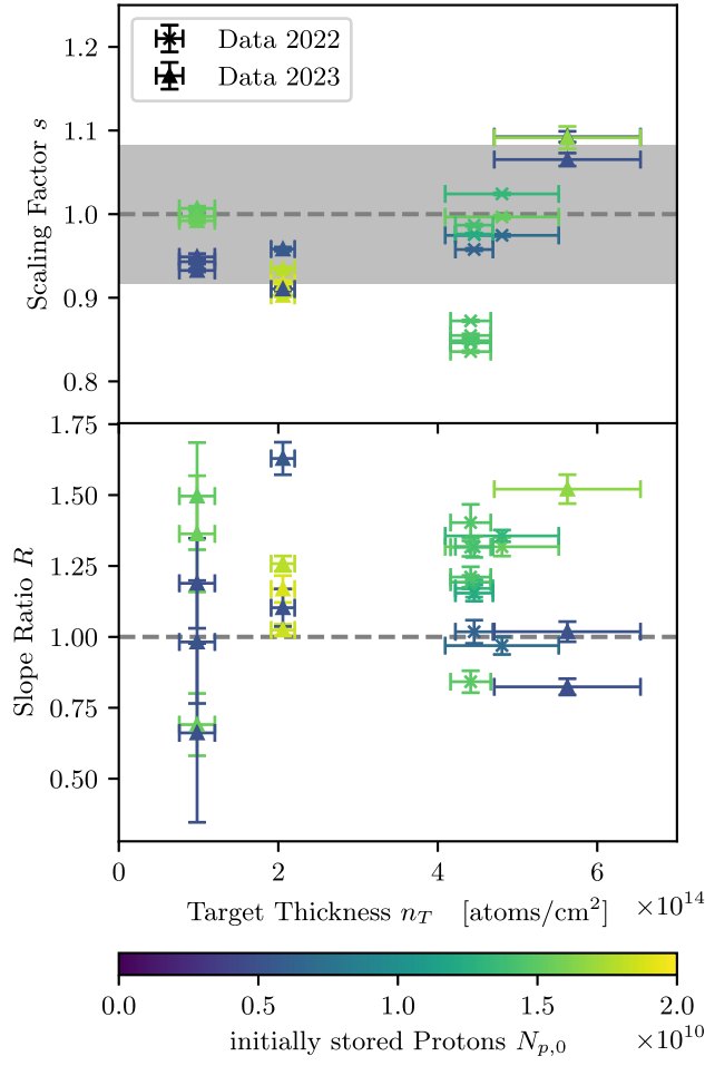
FIG. 18. Results for the linear fit to the momentum spread during a long cycle. Only data with a beam loss of at least 5% are displayed, so that the slope can be determined precisely. Top: scaling parameters to scale the fit function from Sec. V as the starting point of a linear function to the data of the long cycles. The gray error band visualizes the additional uncertainty factor k around the expected scaling factor of 1. Bottom: slope ratio R of the linear fit function to the function ss_{br}g(n_T, N_p) at the point (n_T, N_{p,0}) . If the linear function would be a tangent, the value should be 1 as indicated by the dashed line.
