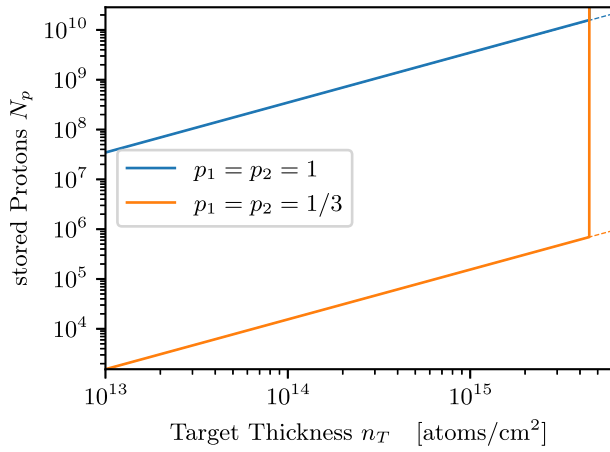
FIG. 11. Optimum combinations of target thickness and beam intensity, which result in the smallest equilibrium momentum spread for that luminosity with p_1 = p_2 = 1/3 and p_1 = p_2 = 1 . Once the target thickness reaches its maximum, which is assumed to be the PANDA design value of 4.5 \times 10^{15} atoms/cm 2 , only the beam intensity can be changed (vertical lines). This deviation from the optimum combination (dashed lines) will result in a stronger increase of the momentum spread as shown in Fig. 12.
