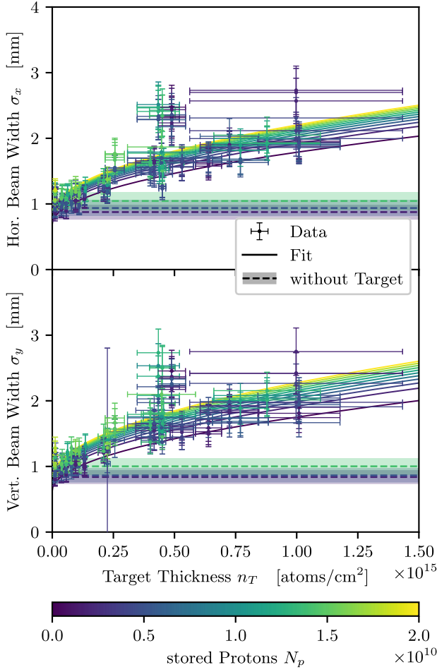
FIG. 13. Equilibrium horizontal (top) and vertical (bottom) beam widths as a function of the target thickness and the number of stored particles in COSY with a power law fit [Eq. (12)] with p_1 = p_2 = 1/2 . The data of the beam times in 2021 and 2022 are scaled by 1/s_{bt} , which is determined by the fit. Additional data taken without a target are shown as horizontal lines. The additional uncertainty [Eq. (16)] is included in the vertical error bars and error bands.
