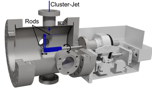
FIG. 5. CAD drawing of the absolute thickness monitor system (AMS) that is installed at the \bar{\text{P}}\text{ANDA} cluster-jet target setup at COSY. The two rods scan through the cluster jet one after the other to get beam profiles in two dimensions. Clusters hitting these rods cause a pressure increase that is recorded and that can be converted into an absolute target thickness.
