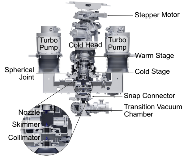
FIG. 1. CAD drawing of the \bar{\text{P}}\text{ANDA} cluster-jet target source. Ultrapure hydrogen gas enters the target and is cooled within the copper pipe windings around the warm and cold stages of the two-stage cold head. The gas is pressed under high pressure of up to 20 bar and temperatures down to 20 K through a convergent-divergent de Laval nozzle. The resulting cluster jet is separated from residual gas and shaped by a circular skimmer and a rectangular collimator. Gas remaining inside the skimmer or collimator chamber is pumped away by a powerful pumping station and two turbomolecular pumps.
