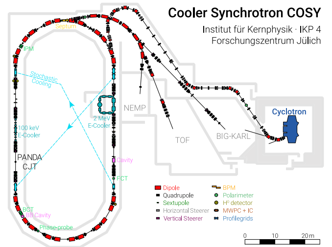
FIG. 3. Plan of the COoler SYnchrotron (COSY). Proton and deuteron beams can be injected from the cyclotron JULIC and are then accelerated to their final momenta of up to 3.7 GeV/c. This beam can then be used by internal experiments or it can be extracted and guided toward the external experimental areas. The PANDA cluster-jet target is installed at the former WASA experimental area on the left side. Additionally, the stochastic cooling system for the HESR is installed at COSY with the pickup tank on the lower right of the ring and the kicker on the upper left.
