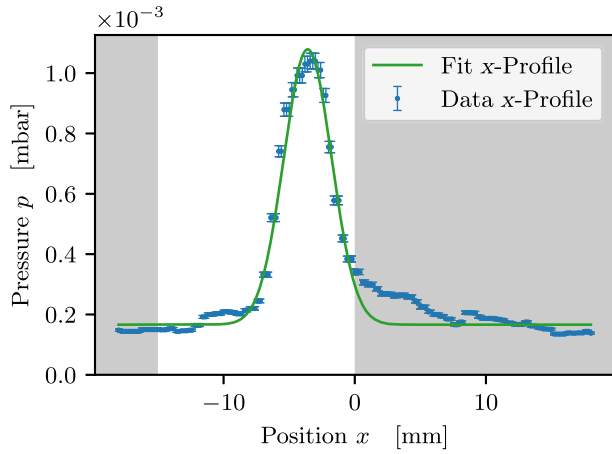
FIG. 6. Target profile recorded with the target operating at 23 K and 18 bar with a record target thickness of (3.14 \pm 0.17) \times 10^{15} atoms/cm 2 . The data in the gray area are not included in the fit to avoid the influence of the asymmetric shape.
