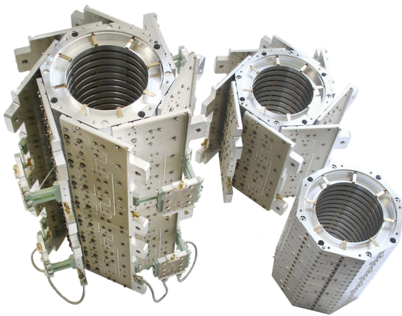
FIG. 2. Ring-slot coupler stacks for the HESR stochastic cooling system. The smaller stacks on the right are shown without and with combiner boards. Two of them are then combined to the final stack size on the left [29].
