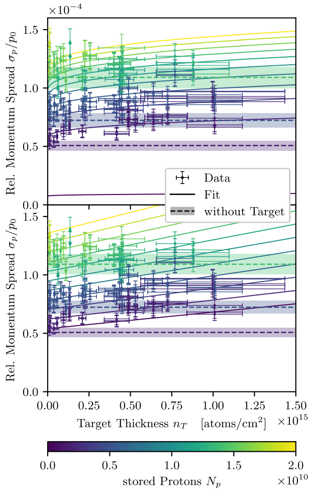
FIG. 10. Equilibrium momentum spread as a function of the target thickness and the number of stored particles in COSY with a power law fit [Eq. (12)] with p_1 = p_2 = 1/3 (top) and p_1 = p_2 = 1 (bottom). The data of the beam times in 2021 and 2022 are scaled by 1/s_{bt} , which is determined by the fit. Additional data taken without a target are shown as horizontal lines. The additional uncertainty [Eq. (16)] is included in the vertical error bars and error bands.
