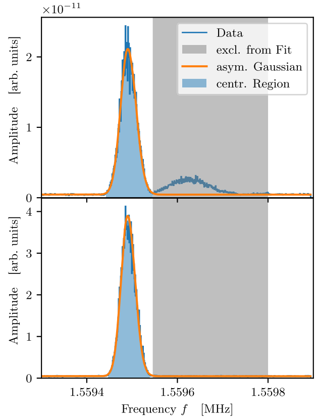
FIG. 8. Recorded Schottky spectra with the target operating at 23 K and 18 bar with a resulting target thickness of (1.00 \pm 0.42) \times 10^{15} atoms/cm 2 (top) and at 32 K and 18 bar with (1.32 \pm 0.05) \times 10^{14} atoms/cm 2 (bottom). In the upper plot, the data show a clear side peak that is excluded (gray area) from the analysis. This cannot be observed at smaller target thickness as shown in the lower plot.
