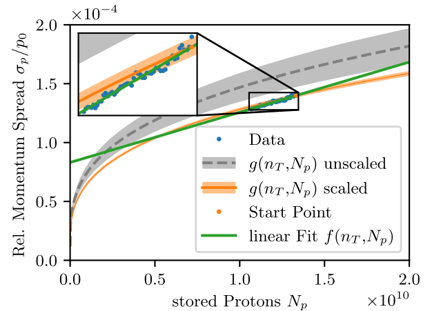
FIG. 17. Momentum spread evolution during a cycle due to the beam intensity reduction recorded with a target thickness of (4.4 \pm 0.3) \times 10^{14} atoms/cm 2 at 28 K and 18 bar. The fit function from Sec. V is scaled and used as the starting point for a linear function as defined in Eq. (24). The gray error band visualizes the additional uncertainty that reflects the manual adjustment of the stochastic cooling that was introduced with the fit. The orange error band, on the other hand, includes the uncertainties of the fit function and the target thickness.
