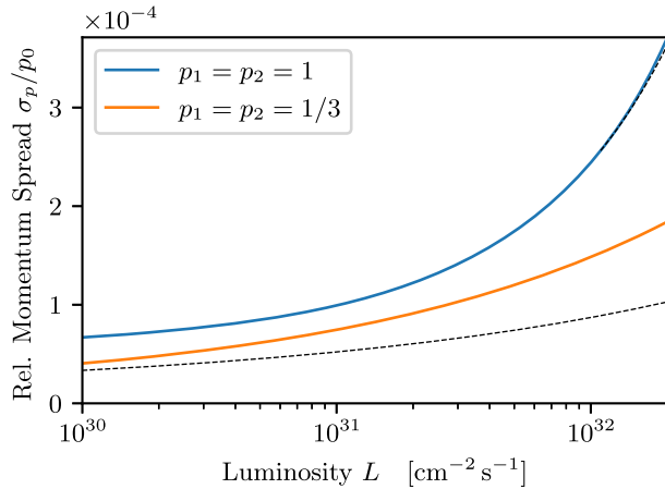
FIG. 12. Momentum spread as a function of the luminosity when operating with the optimum combinations of target thickness and beam intensity. Once the maximum target thickness ( 4.5 \times 10^{15} atoms/cm 2 ) is reached, only the beam intensity can be changed, which will result in a stronger increase of the momentum spread and a deviation from the optimum (dashed lines). For p_1 = p_2 = 1 , this point is reached at a luminosity of approximately 1.1 \times 10^{32} cm -2 s -1 , while for p_1 = p_2 = 1/3 , it is already reached at around 4.9 \times 10^{27} cm -2 s -1 .
