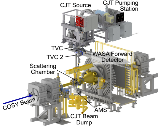
FIG. 4. CAD drawing of the \bar{\text{P}}\text{ANDA} cluster-jet target (CJT) setup at COSY. The target source is installed on top of the concrete ceiling of the COSY tunnel at the location of the former WASA experiment. The WASA central detector was removed to make space for a larger scattering chamber, an absolute thickness monitor system (AMS), and the target beam dump. While the distance between target source and the interaction point is in \bar{\text{P}}\text{ANDA} geometry, the distance to the beam dump is reduced due to space constraints. Downstream of the interaction point, the WASA forward detector is located and still operational. It was used to find the perfect overlap of the COSY beam and the target by monitoring the rate.
