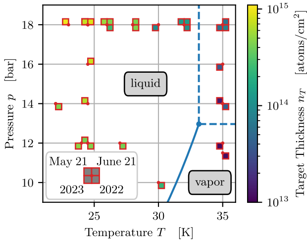
FIG. 7. Target settings with the resulting target thicknesses used during the beam quality measurements in the phase diagram of hydrogen. The solid blue line corresponds to the vapor pressure curve, and the dashed lines mark the region of supercritical hydrogen. The four quadrants correspond to the three beam times with the 2021 beam time divided into two parts in May and June.
