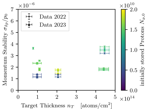
FIG. 16. Momentum stability for different target settings and beam intensities. The initial beam intensity was determined shortly before the target was turned on.
