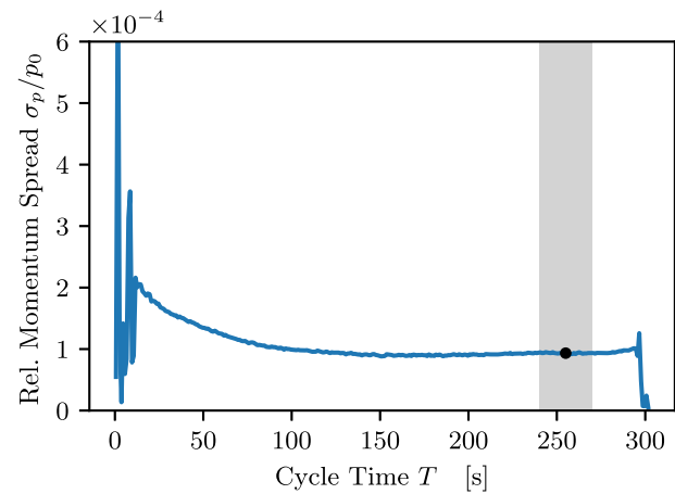
FIG. 9. Relative momentum spread evolution during a cycle with a target thickness of (1.32 \pm 0.05) \times 10^{14} atoms/cm 2 at 32 K and 18 bar. The equilibrium value is extracted as mean at the end of the cycle (gray area).
