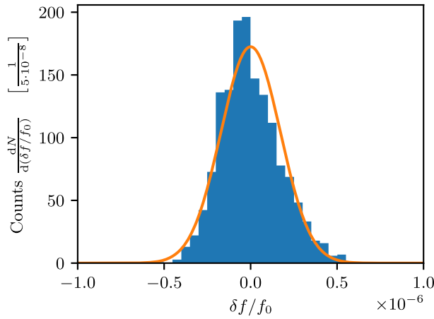
FIG. 15. Histogram showing the relative deviation of the mean frequency of the Schottky spectra from the nominal frequency during a long cycle. The data were recorded with the target operating at 28 K and 18 bar with a target thickness of (4.4 \pm 0.3) \times 10^{14} atoms/cm 2 . The orange line shows a Gaussian with the same center, area, and standard deviation as the histogram.
