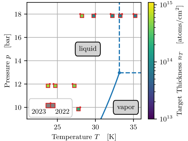
FIG. 14. Target settings with the resulting target thicknesses used during the beam stability measurements in the phase diagram of hydrogen. The solid blue line corresponds to the vapor pressure curve, and the dashed lines mark the region of supercritical hydrogen.
