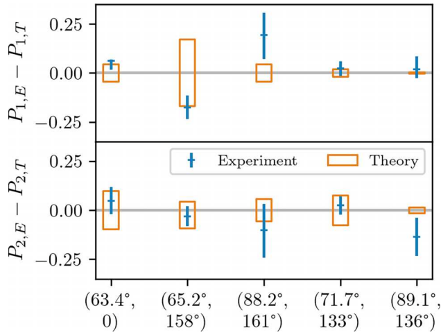
FIG. 5. Difference of the measured Stokes parameters of the Rayleigh scattered photons and the theoretical predictions from the S -matrix approach. The length of the blue error bars is given by the root sum squared of the individual experimental uncertainties, the theoretical uncertainty is indicated by the orange boxes.
