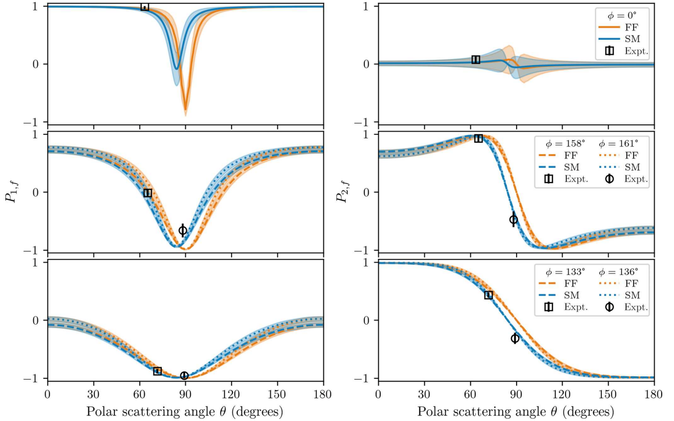
FIG. 4. Stokes parameters P_{1,f} (left) and P_{2,f} (right) of the Rayleigh-scattered photon beam for both experimental data (black errorbars) and theoretical models based on a modified form factor with angle-independent anomalous scattering factor [30] (orange) and on the S matrix [16] (blue), the shaded area shows the corresponding uncertainties. The theory curves are shown for an extended detector. Each row represents results for similar azimuthal scattering angles, top: \phi = 0^\circ , middle: \phi \approx 160^\circ , bottom: \phi \approx 135^\circ .
