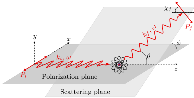
FIG. 1. Geometry of Rayleigh scattering of a linearly polarized photon beam. The incident photons propagate along the z axis. The polarization plane of the incident photon beam is chosen as reference. The wave vectors of the incident and scattered photons k_i and k_f span the scattering plane. The scattered photon direction is defined by the polar and azimuthal scattering angles \theta and \phi . The polarization vector of the scattered photons is defined with respect to the scattering plane with the polarization angle \chi_f .
