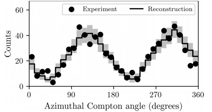
FIG. 3. Azimuthal distribution of Compton scattering within the detector positioned at \theta = 65.2^\circ , \phi = 158^\circ . The events are limited to x rays being Rayleigh scattered by the gold target. For a better visual representation, the distribution was corrected for geometrical and binning effects. Additionally, a reconstruction of the azimuthal distribution is displayed with a probability interval of 0.68 (shaded area).
