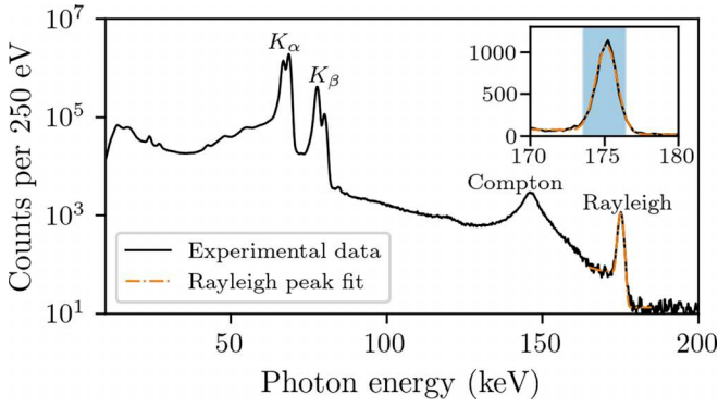
FIG. 2. Energy-resolved spectrum of 175 keV photons scattered by gold, obtained from single-hit events within the Compton polarimeter positioned at \theta = 65.2^\circ , \phi = 158^\circ . The spectrum is not corrected for the efficiency of the detector. The inset plot shows a zoom to the Rayleigh peak, the shaded area highlights the area of interest for the polarization analysis.
