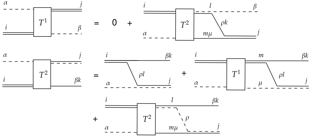
Figure 6. Integral equations for the coupled-channel ( T_{cc}^*D and T_{cc}D^* ) scattering amplitudes. Here, the single solid (dashed) line represents D^* ( D ) meson, and the double solid (solid-dashed) line represents the D^*D^* ( DD^* ) dimer T_{cc}^* ( T_{cc} ).
