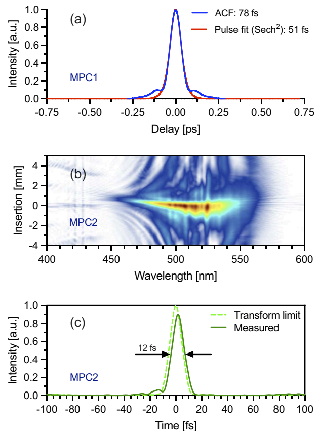
Figure 2. (a) Measured autocorrelation trace of the pulses after the MPC1 stage. (b) measured d-scan trace and (c) retrieved pulse shape of the MPC2 stage.
